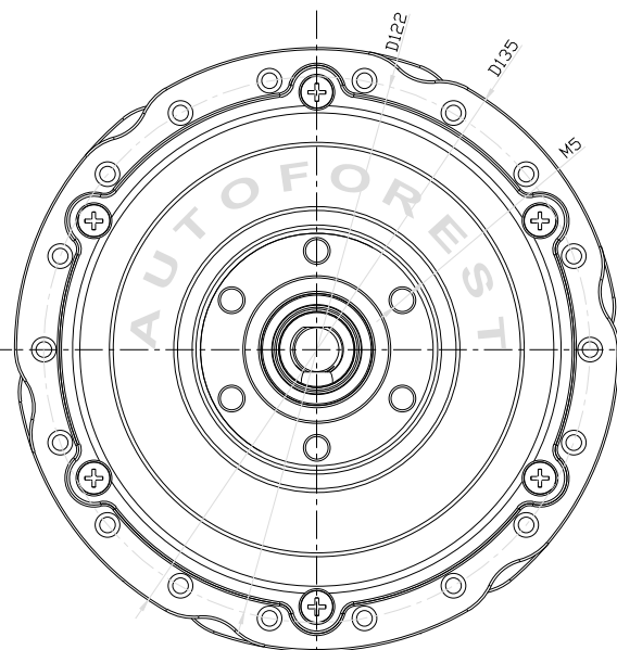
LHS VIEW
