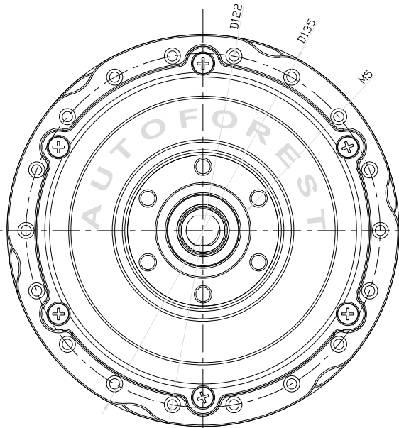
LHS VIEW
