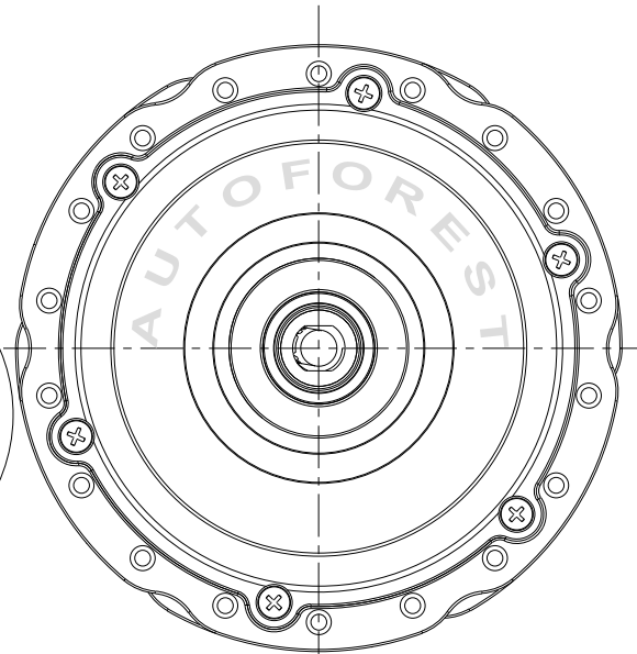
RHS VIEW
