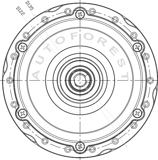
RHS VIEW
